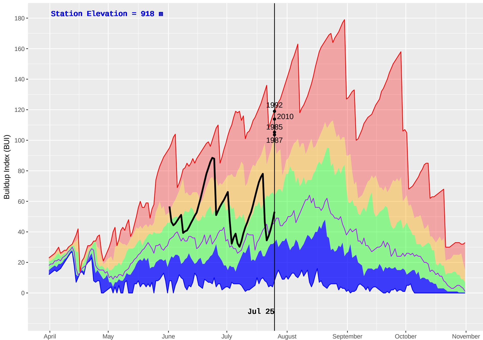
AUGIER LAKE (167) : Historical (1984–2016) and Current (2018) Noon Buildup Index (BUI)
