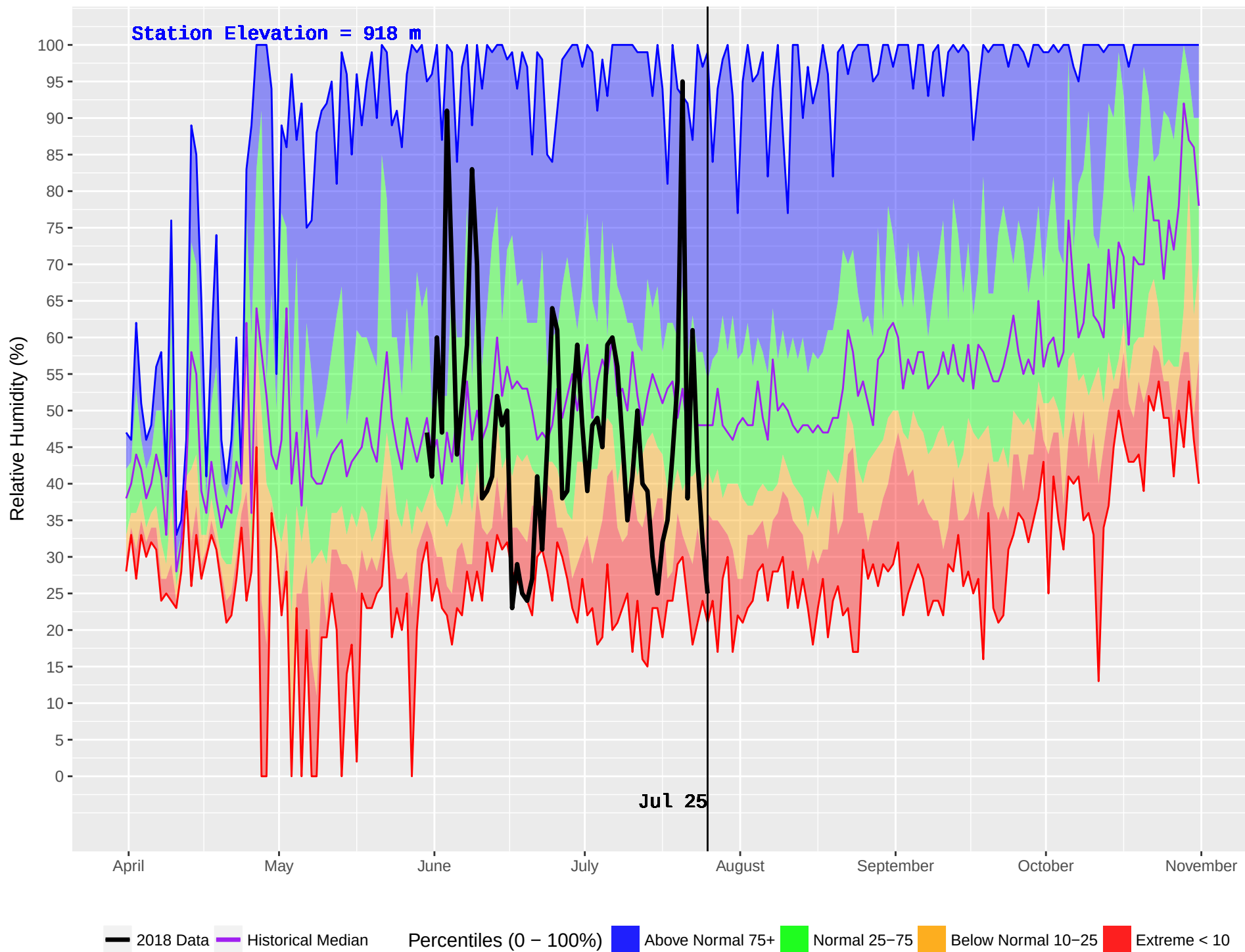
AUGIER LAKE (167) : Historical (1984–2016) and Current (2018) Noon Relative Humidity
